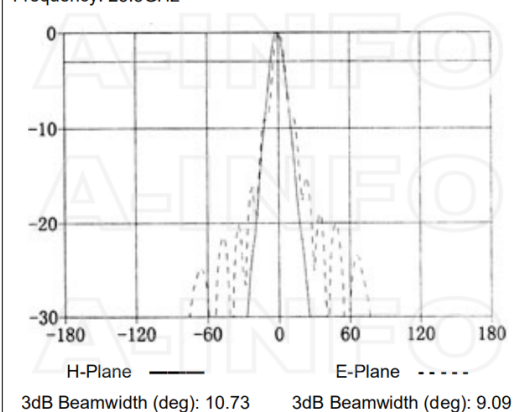
Frequency: 25.5GHz
