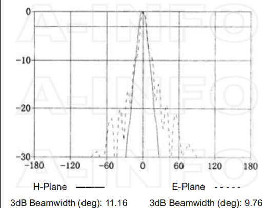
Frequency: 23.5GHz
