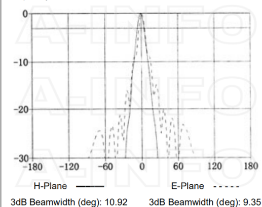
Frequency: 24.5GHz
