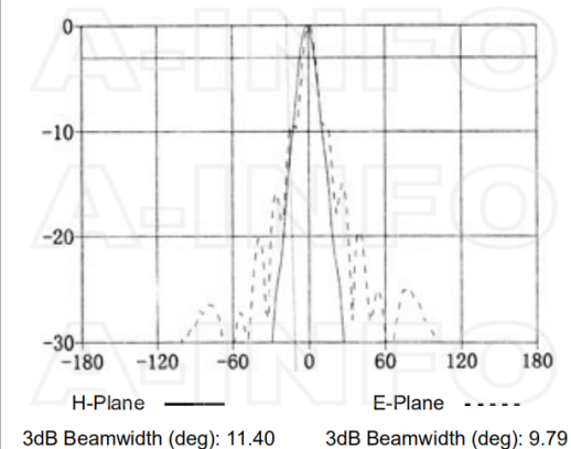
Frequency: 23.0GHz
